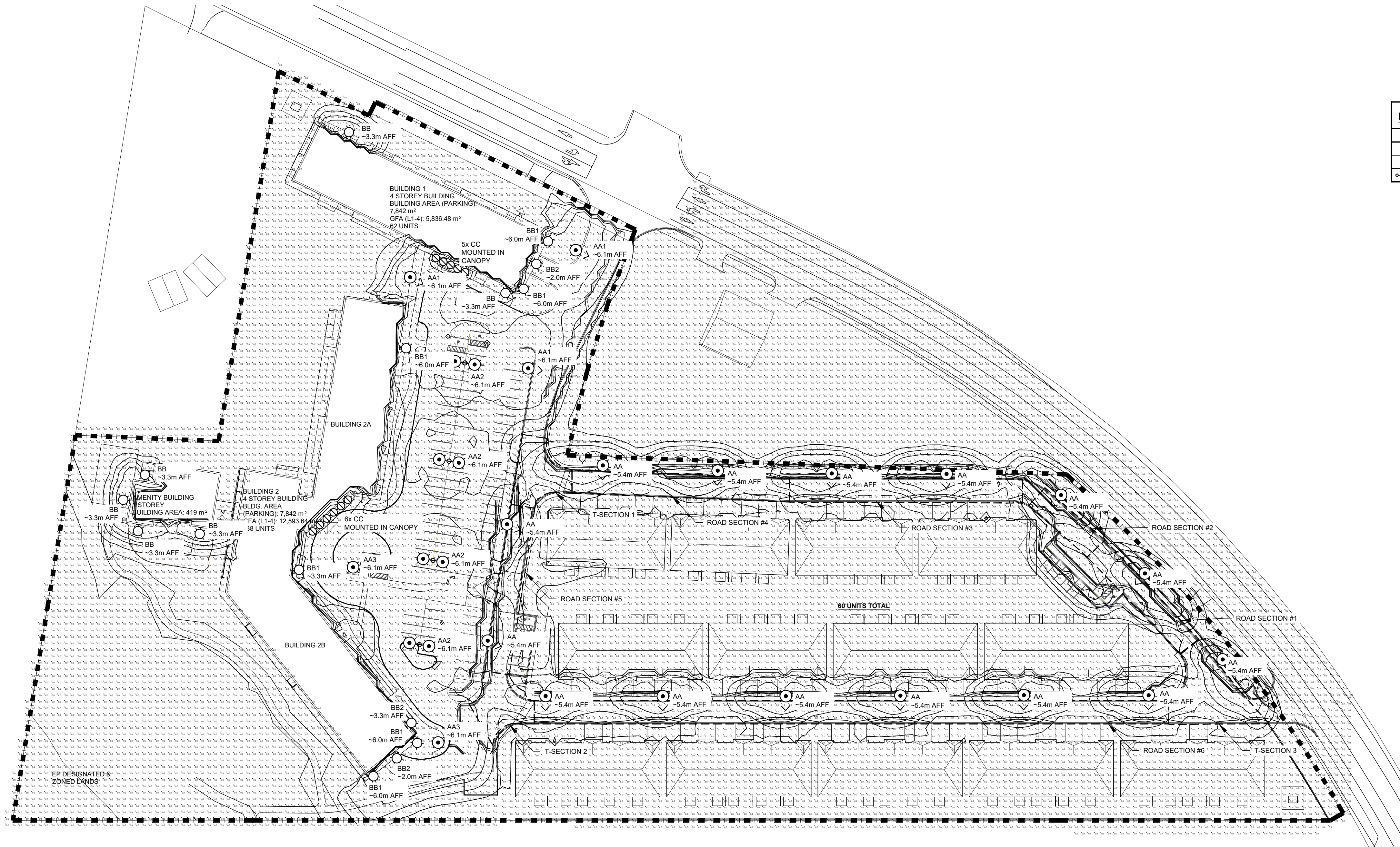
1 SITE PLAN SLP-1 SCALE: 1:750
