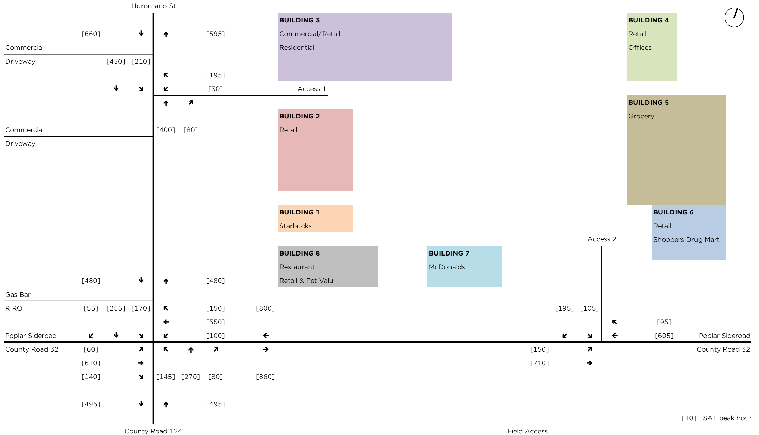
THE GATEWAY CENTRE - TRANSPORTATION IMPACT STUDY Figure 20B: Traffic Volumes - 2040 Total Saturday
