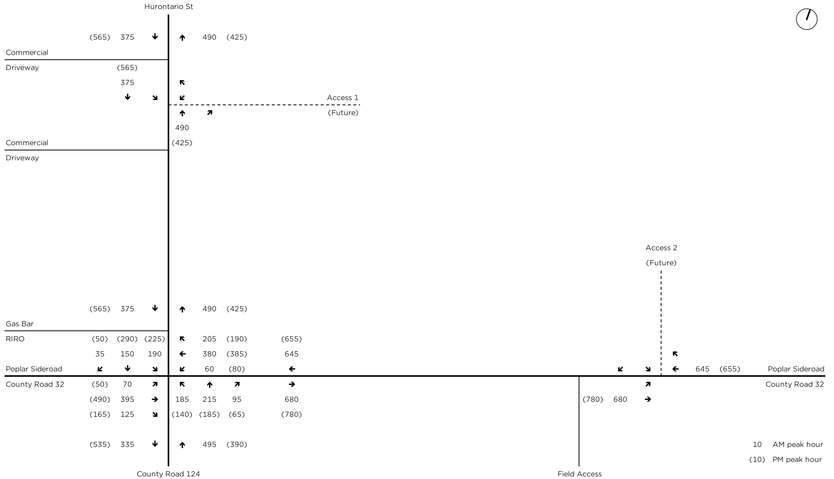
THE GATEWAY CENTRE - TRANSPORTATION IMPACT STUDY Figure 8A: Traffic Volumes – 2030 Background Weekday
