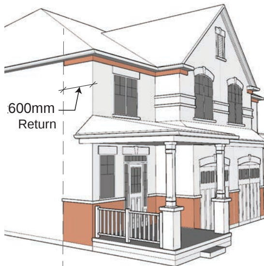
Detail of Material Return on Side Walls
