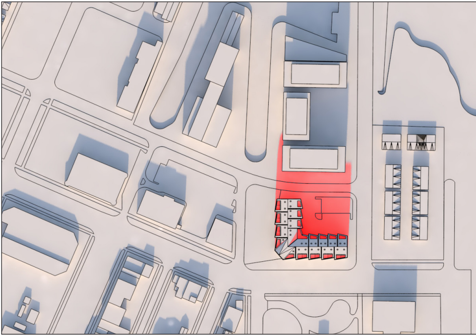
December 21 - 10.18 hrs
