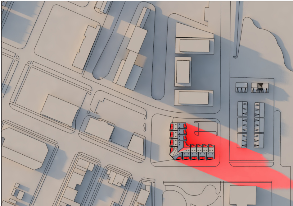
September/March 21 - 18.18 hrs
