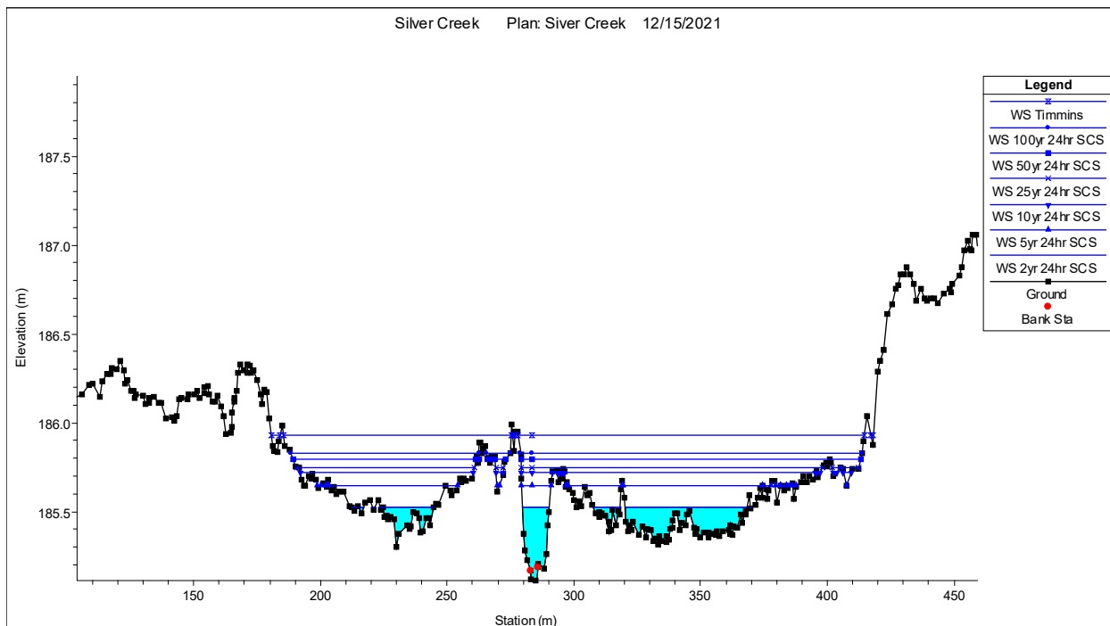
Figure 7-8 HEC-RAS Section 1767.4
