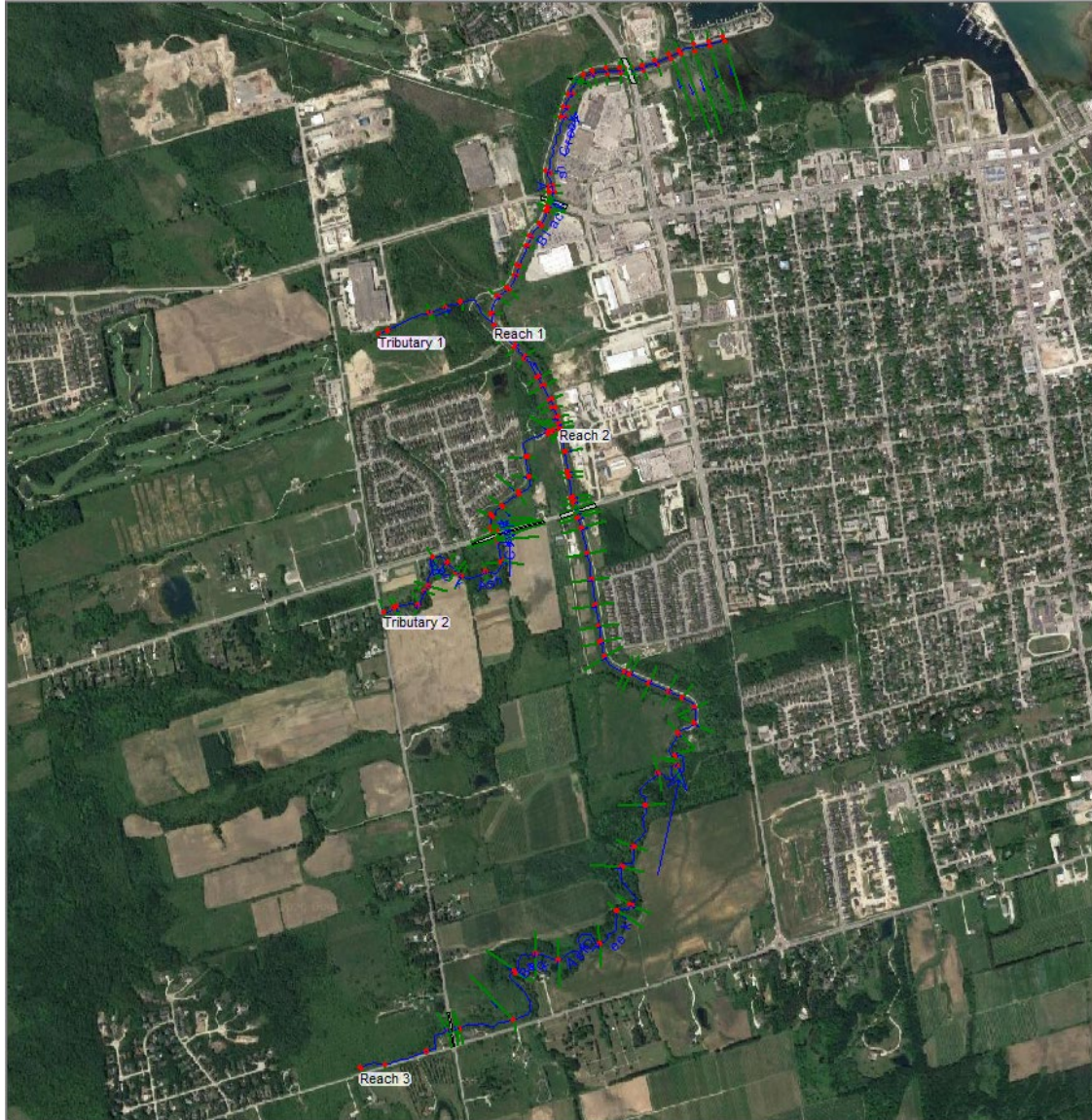
Figure 5-1 Black Ash Creek HEC-RAS Model Layout
