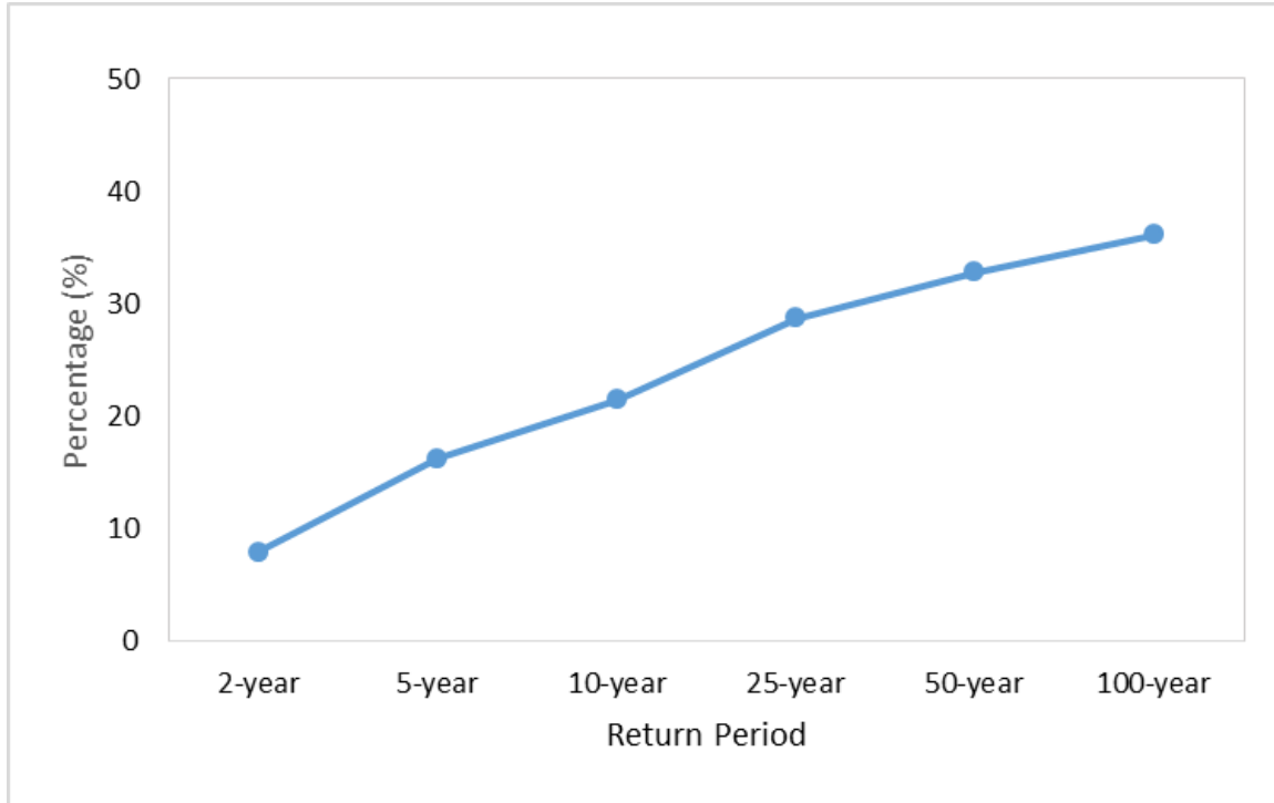
Figure 7-24 Percentage of Nodes Surcharged, Urban Town Centre
