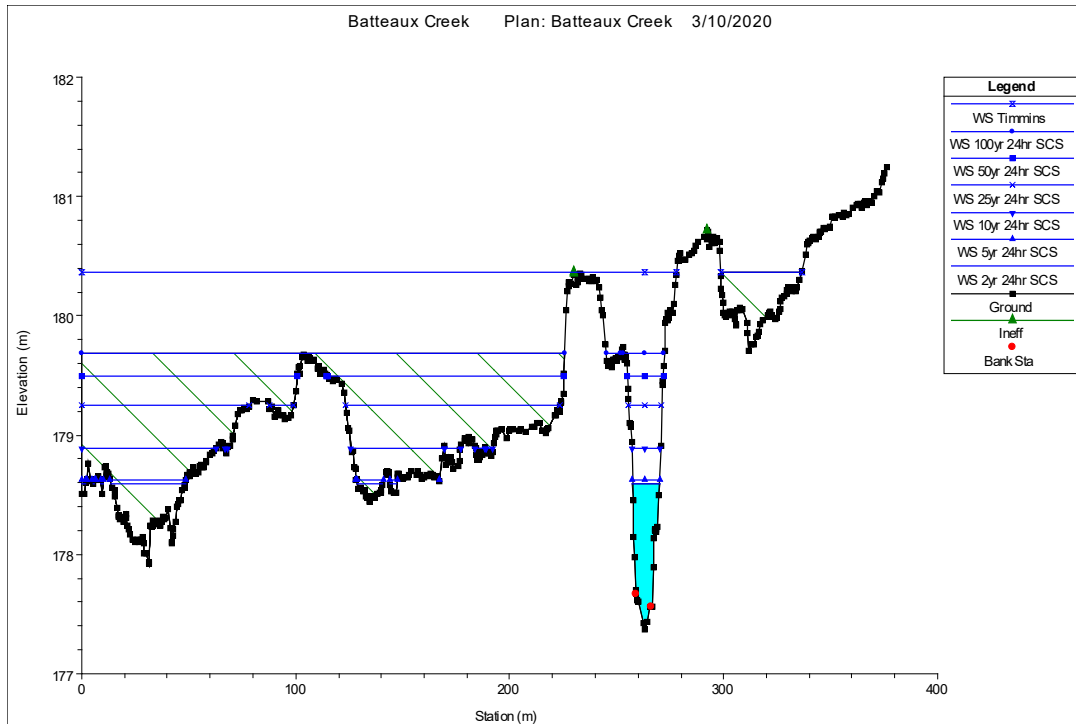
Figure 7-22 HEC-RAS Section 324.2
