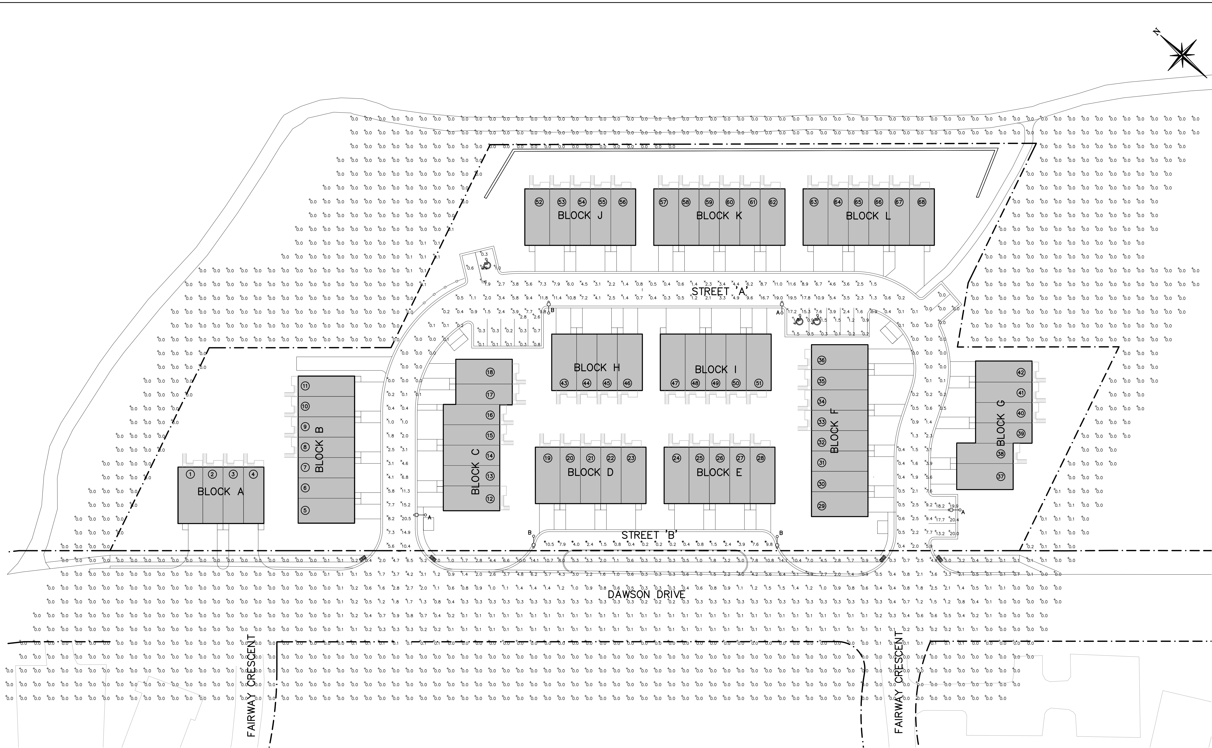
SITE PLAN – PHOTOMETRIC SCALE: 1:400
